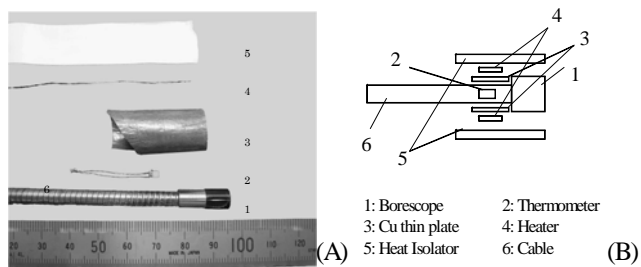
Fig.1 (A) Photo and (B) schematic view of a temperature controlled video bore scope.
