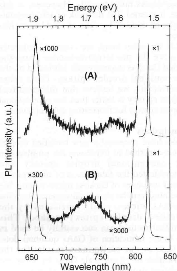
Fig.2 Photoluminescence spectra of buried structures observed at 15 K. Al composition of buried microcrystals are 3 % (A) and 10 % (B).
