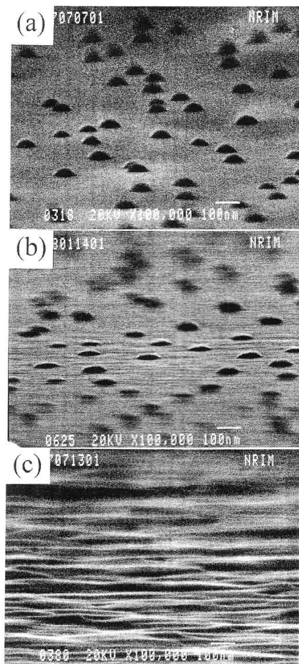
Fig.1 Surface morphologies of the samples; (a) \text{Ga}_{0.90}\text{Al}_{0.10} droplets, (b) \text{Ga}_{0.90}\text{Al}_{0.10}\text{As} microcrystals just before overgrowth, and (c) after the growth of overlayer.
