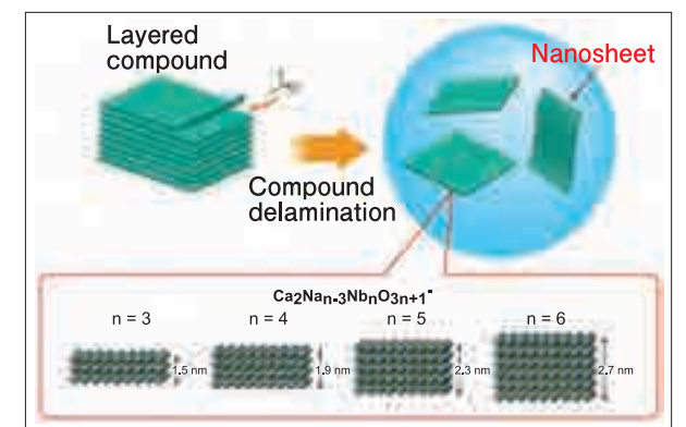
Soft-chemical exfoliation process to produce perovskite type oxide nanosheets.
