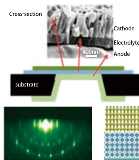
Top: Solid oxide fuel cell
