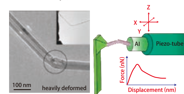
Mechanical properties of a BN nanotube measured inside TEM
