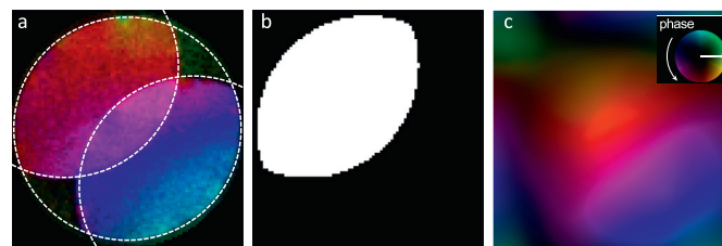
Fig. 2. Schematic illustration of the Wigner distribution deconvolution (WDD) procedure. (a) The complex 4D dataset G(\mathbf{K}_f, \mathbf{Q}_p) at a single probe spatial frequency \mathbf{Q}_p (as shown in Fig. 1d) shows beam interferences at the detector plane between the undiffracted central beam and two diffracted first order beams, as indicated by dashed circles. (b) The Fourier transform of the Wigner distribution function of the probe function, i.e., A(\mathbf{K}_f)A^*(\mathbf{K}_f + \mathbf{Q}_p) . In the case of zero lens aberration, it's the overlapping region of two top-hat aperture functions. After deconvolving (b) from (a), the Fourier transform of the Wigner distribution function of the object, i.e., \Psi(\mathbf{K}_f)\Psi^*(\mathbf{K}_f - \mathbf{Q}_p) is shown in (c). The modulus and phase are combined in (a) and (c), with the phase represented by color and modulus by brightness, as indicated on the color wheel scale. Figure (a)–(c) are shown in the detector \mathbf{K}_f plane, with \mathbf{K}_f = 0 located at the center of each figure.
