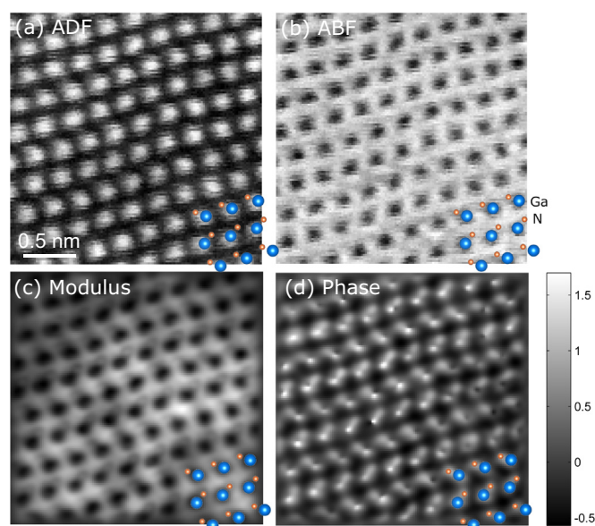
Fig. 6. Simultaneous ADF, synthetic ABF, and the reconstructed modulus and phase of bulk GaN imaged along [211̄0]. The probe forming aperture is around 14.4 mrad, and the synthetic ABF has a collection angle of 7.2–14.4 mrad. The diffraction patterns were recorded using 66 × 264 detector pixels at 4000 frames per second speed.
