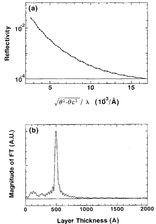
Fig.2 Thickness determination of SiO 2 layer (50.1 nm) formed on Si substrate by Fourier transform of X-ray reflectivity with 8 keV synchrotron photons. (a) X-ray reflectivity plotted as a function of q'_z considering critical angle correction. (b) Magnitude of Fourier transform of the oscillating part extracted from the curve (a). (Reproduced with permission from [21], Fig.2)
