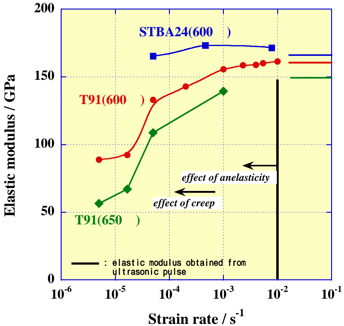
Fig. Effect of strain rate on elastic modulus obtained from tensile test.
